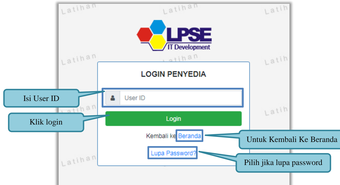
Gambar 5. Form Login 1
